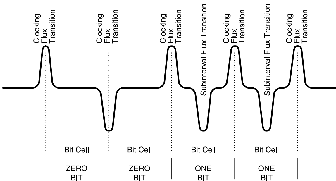
Figure 2-1. Bit Cell - Flux Transition
